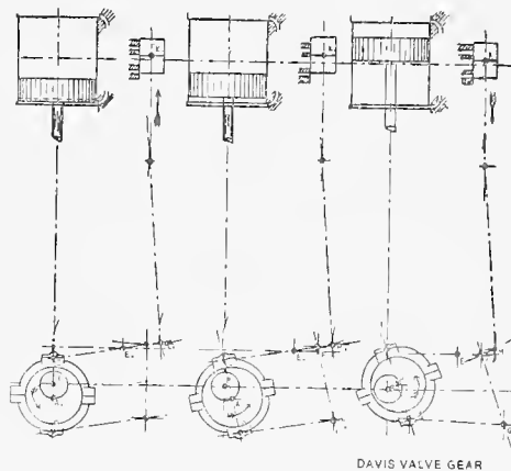
FIG. 2. FIG. 3. FIG. 4 The Davis Radial Valve Gear.
